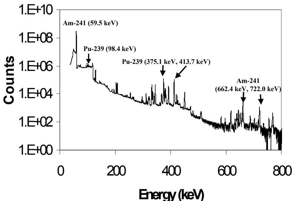
Figure 45 Plutonium spectrum collected for 48 hours from a distance of 15.5 cm using the LN 2 HPGGe detector
