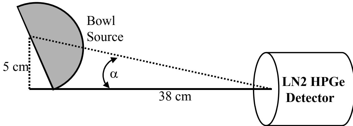
Figure 34 Side view of the geometry with the bowl source and the LN 2 HPGе detector
